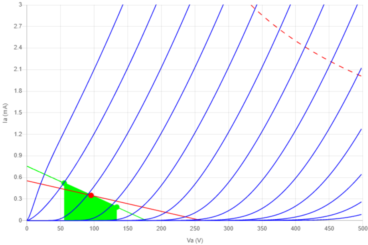
Anode Characteristic Graph: 12AX7 - www.vtadiy.com
